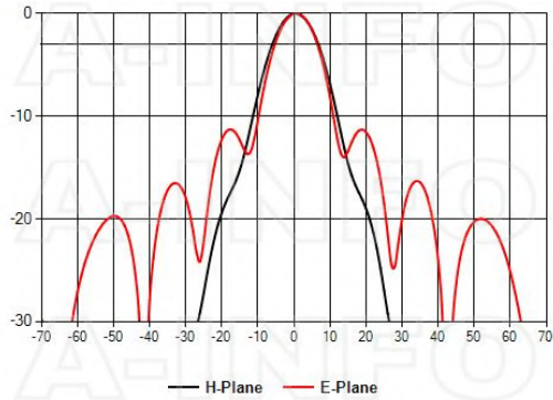
Frequency:18.000GHz
