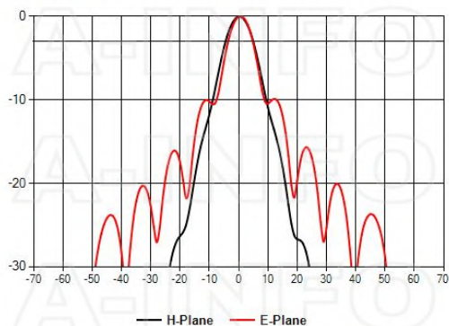
Frequency:26.000GHz
