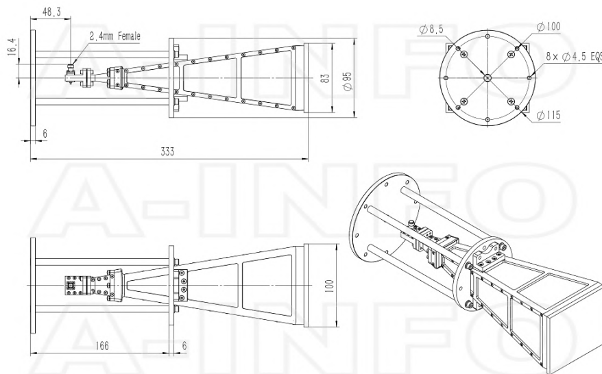
2.4mm-Female Output with Round Mounting Bracket & Radome (Option, P/N: LB-180400-25- MB2 & LB-180500-25-C-2.4FSPO, Outdoor Application)
