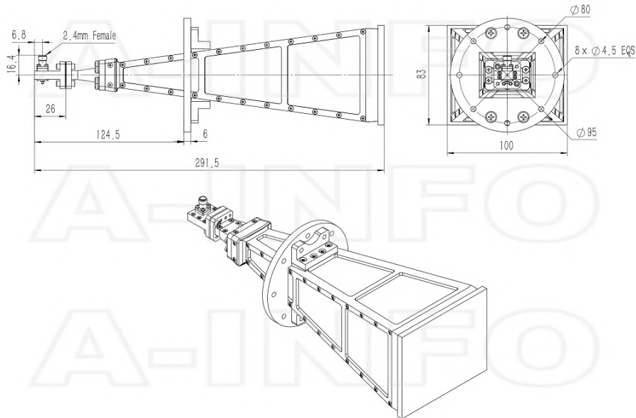
2.4mm-Female Output with Radome (Option, P/N: LB-180500-25-C-2.4FSPO, Outdoor Application)
