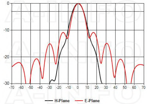
Frequency:20.000GHz
