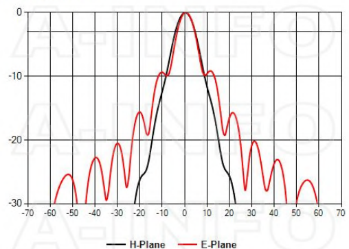
Frequency:28.000GHz
