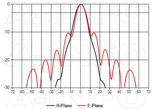
Frequency:24.000GHz
