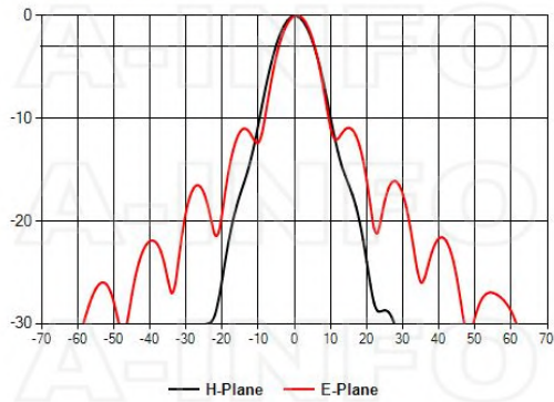
Frequency:22.000GHz
