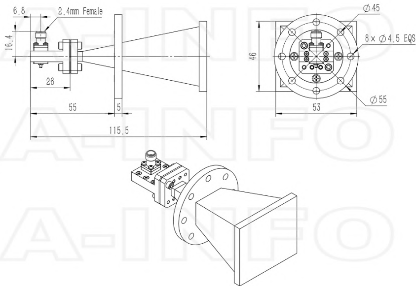
2.4mm-Female Output with Radome (Option, P/N: LB-180500-20-C-2.4FSPO, Outdoor Application)
