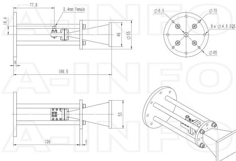
2.4mm-Female Output with Round Mounting Bracket & Radome (Option, P/N: LB-19-25-MB2 & LB-180500-20-C-2.4FSPO, Outdoor Application)
