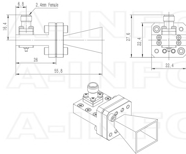
2.4mm-Female Output (P/N: LB-180500-10-C-2.4F)
