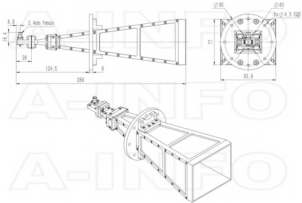
2.4mm-Female Output (P/N: LB-180400-25-C-2.4F)
