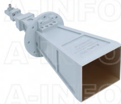
LB-180400-25-C-KF Multi Octave Horn Antenna 18-40GHz 25dB Gain 2.92mm Female
