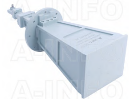
LB-180400-25-C-KFSPO Multi Octave Horn Antenna 18-40GHz 25dB Gain 2.92mm Female
