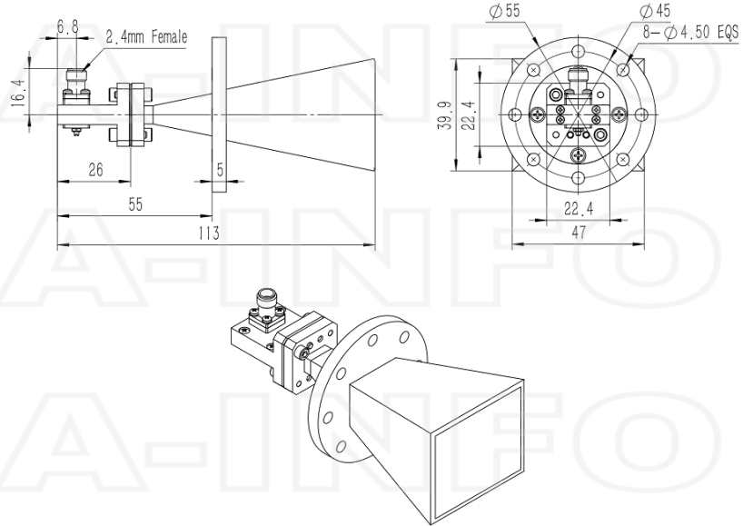
2.4mm-Female Output (P/N: LB-180400-20-C-2.4F)
