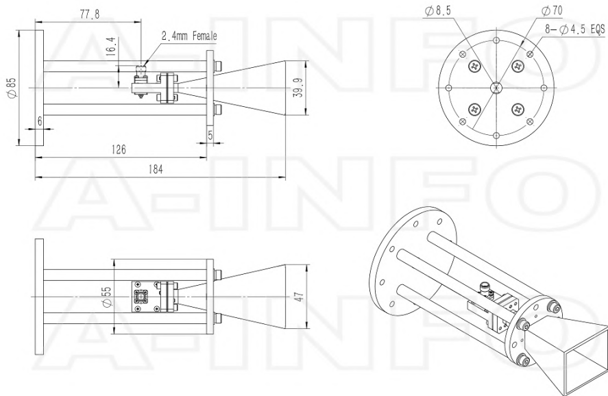
2.4mm-Female Output with Round Mounting Bracket (Option, P/N: LB-19-25-MB2)
