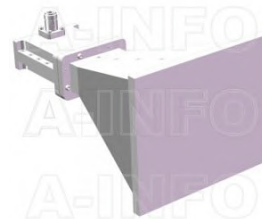
LB-1536-10-C-NFSPO Multi Octave Horn Antenna 1.5-3.6GHz 10dB Gain N Type Female
