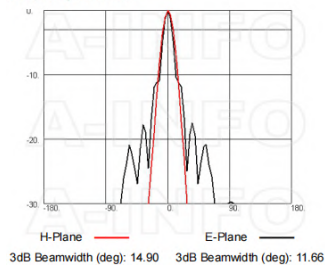
Frequency: 21.0GHz
