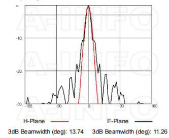
Frequency: 22.0GHz
