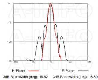
Frequency: 15.0GHz
