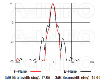
Frequency: 16.0GHz
