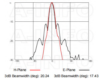
Frequency: 14.0GHz
