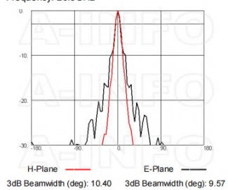
Frequency: 26.5GHz
