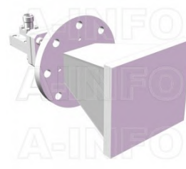
LB-110265-20-C-SFSP0 Multi Octave Horn Antenna 11-26.5GHz 20dB Gain SMA Female
