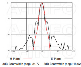
Frequency: 13.0GHz
