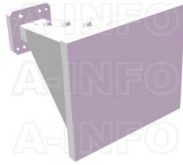
LB-110265-15-ASPO Multi Octave Horn Antenna 11-26.5GHz 15dB Gain Double Ridge Waveguide Interface
