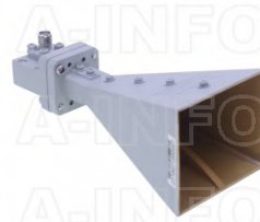
LB-110265-15-C-SF Multi Octave Horn Antenna 11-26.5GHz 15dB Gain SMA Female
