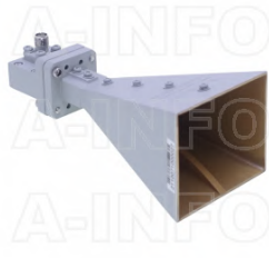
LB-110265-15-C-SF Multi Octave Horn Antenna 11-26.5GHz 15dB Gain SMA Female
