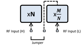
Figure 1: Block diagram of dual input mode is shown. M is the multiplication factor for Low Frequency Mode. N is the multiplication factor for High Frequency Mode.
