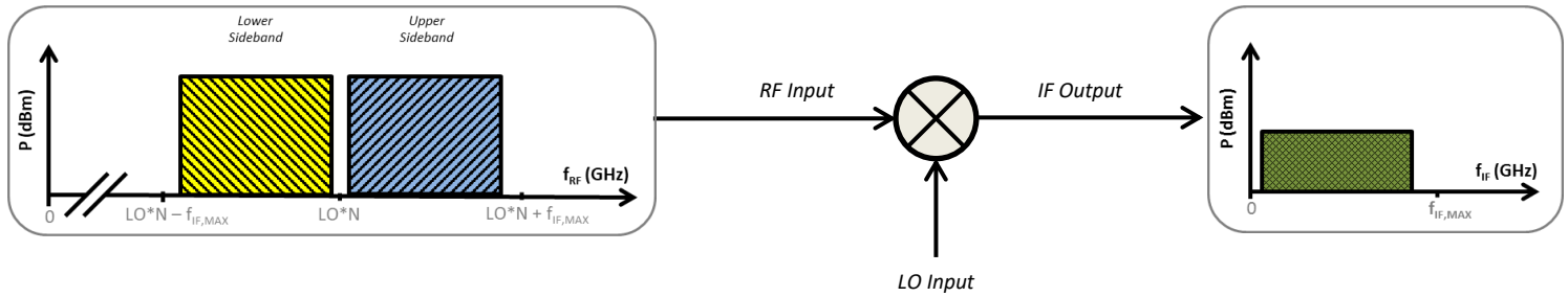
Figure 2: Diagram of block down-conversion is shown.
