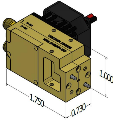
WR6.5
