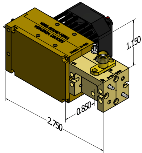
WR1.5, WR1.0
