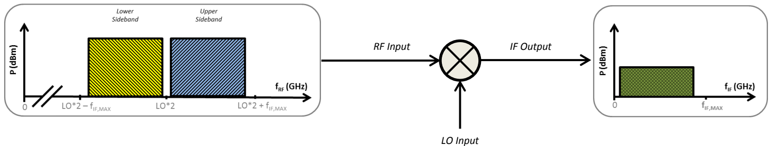
Figure 1: Diagram of block down-conversion is shown.
