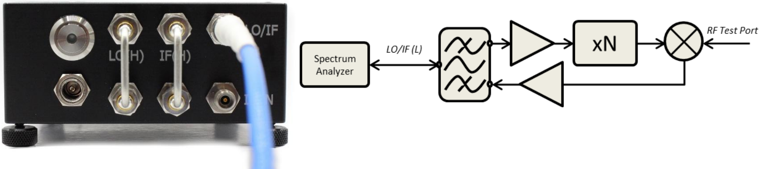
Figure 1: Spectrum Analyzer Extension Proper configuration details for spectrum analyzer extension are shown. The IF Input Port is not used.
