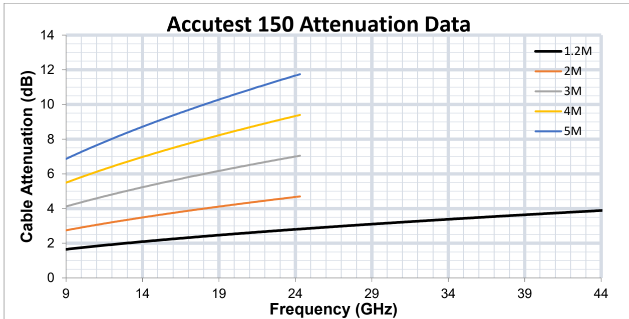
FIGURE 7 - ACCUTEST RF CABLE INSERTION LOSS
