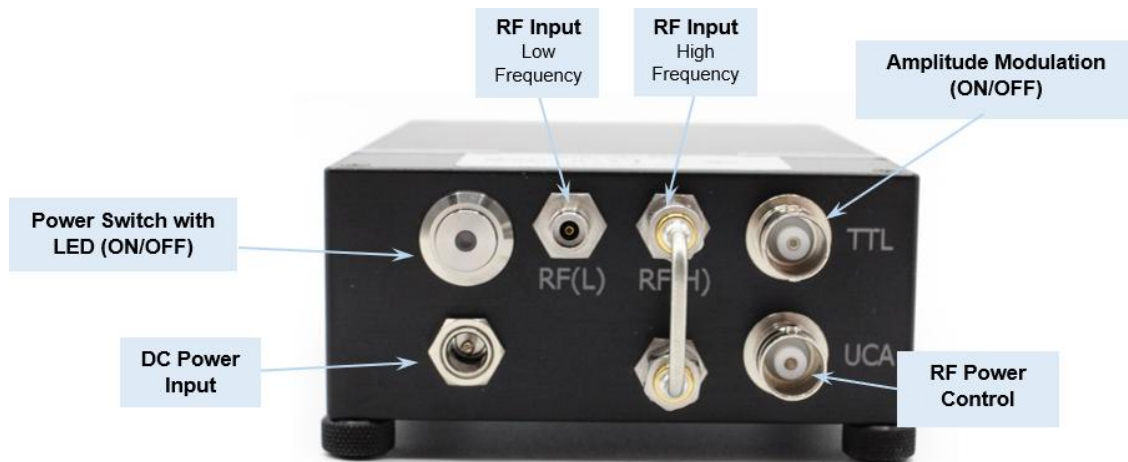
FIGURE 4 - SGX-M REAR PANEL
