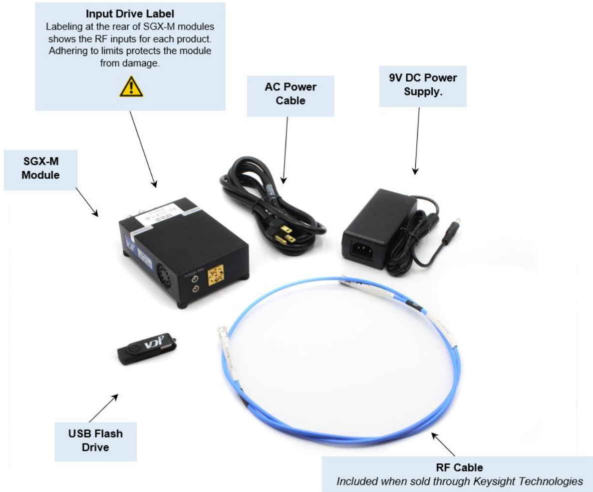
FIGURE 2 - MAJOR COMPONENTS AND ACCESSORIES
