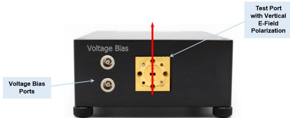
FIGURE 3 - SGX-M FRONT PANEL
