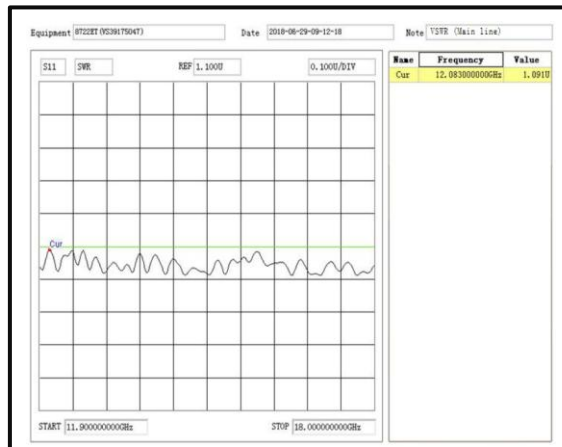
Primary VSWR
