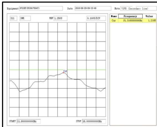
Secondary VSWR
