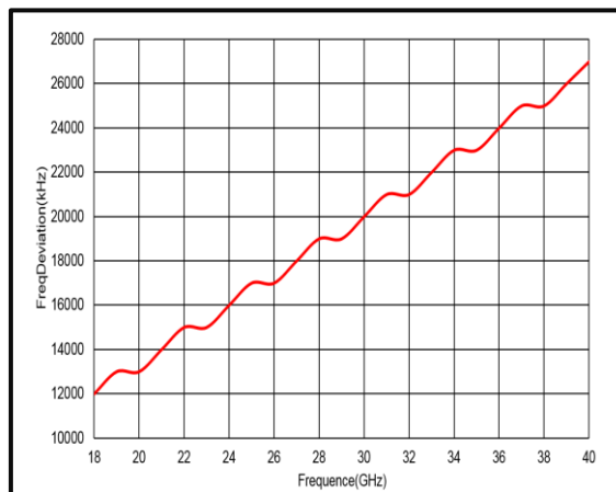
Freq Deviation
