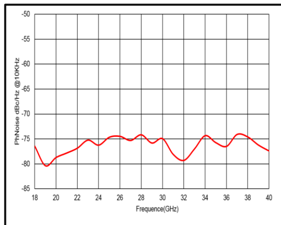
Phase Noise
