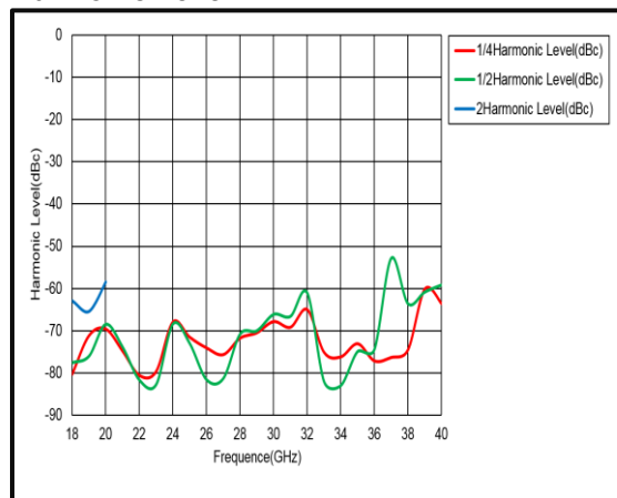
Harmonic Level
