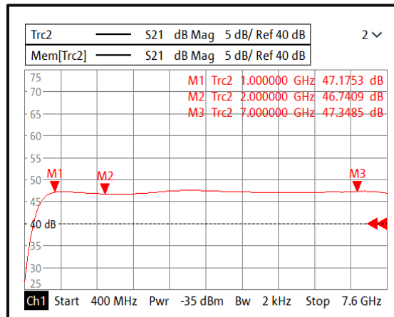
Gain@+85°C
