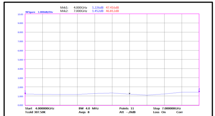
Noise Figure(4GHz-7GHz)
