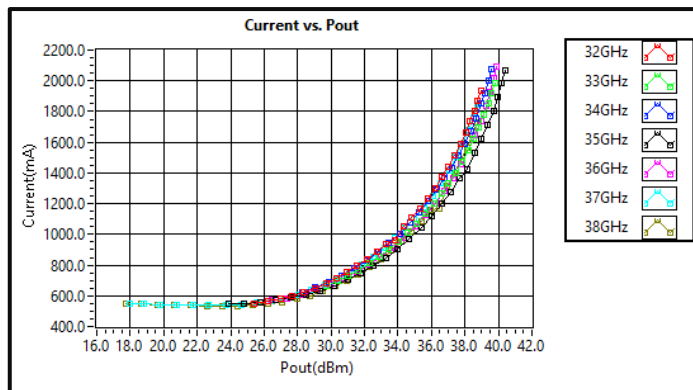
Current vs Output Power (+26VDC)
