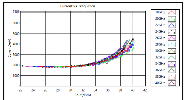
Current vs Output Power (+20VDC)
