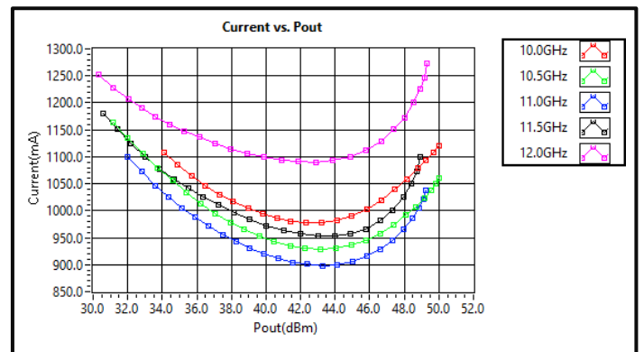
Current vs Output Power *Pulse
