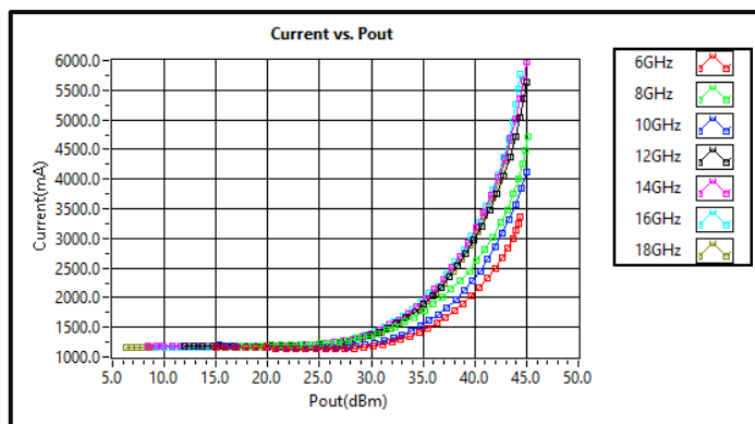
Current vs Output Power (+22VDC)
