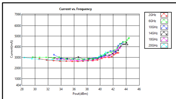
Current vs Output Power (+24VDC)
