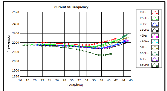
Current vs. Frequency (Pulse)
