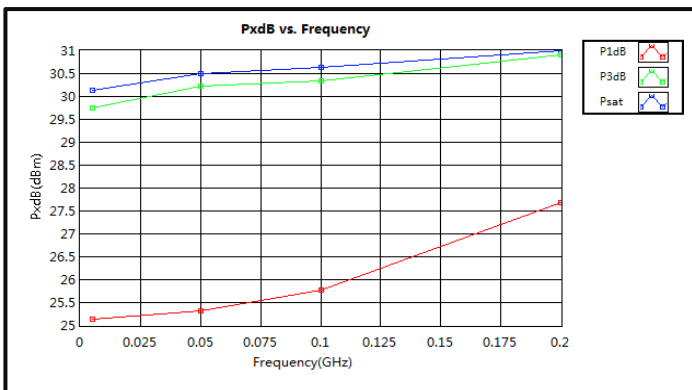
PndB vs. Frequency (5MHz-200MHz)
