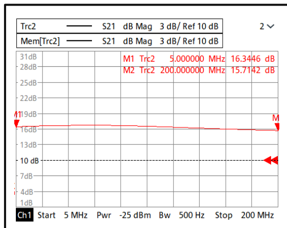
Gain@-40°C (5MHz-200MHz)
