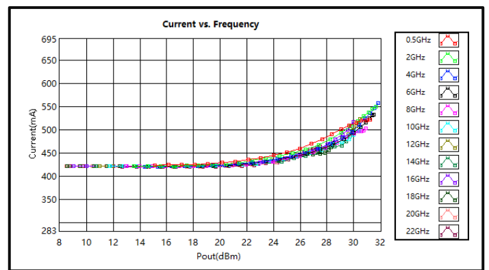
Current vs. Pout (0.5GHz-22GHz)
