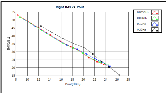
Right IM3 vs. Pout (5MHz-200MHz)
