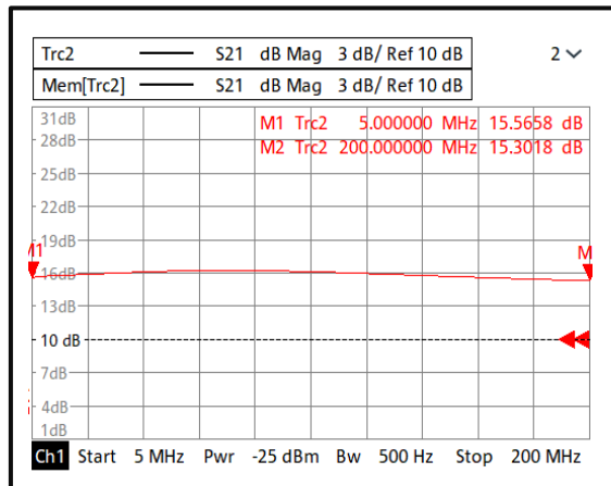
Gain@+25°C (5MHz-200MHz)
