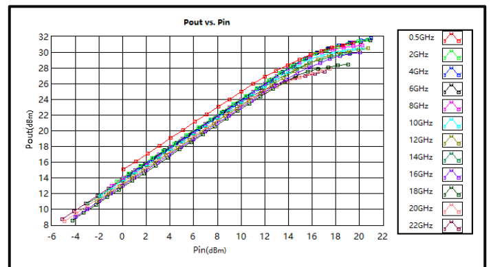
Pout vs. Pin (0.5GHz-22GHz)
