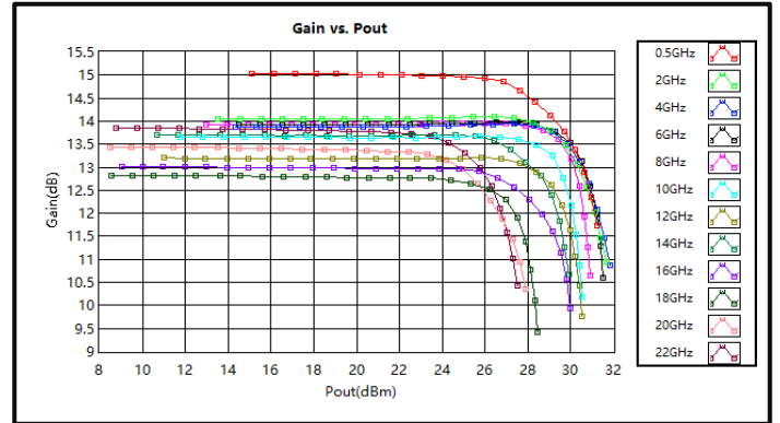
Gain vs. Output Power (0.5GHz-22GHz)
