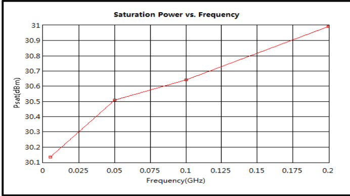
Saturation Power vs. Frequency (5MHz-200MHz)
