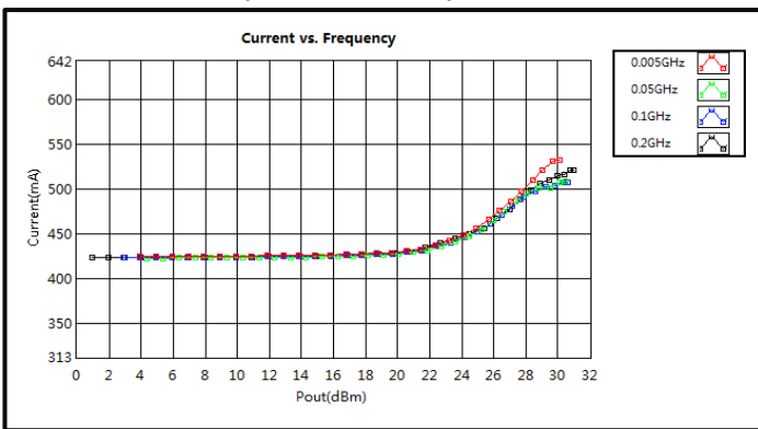
Current vs. Pout (5MHz-200MHz)
