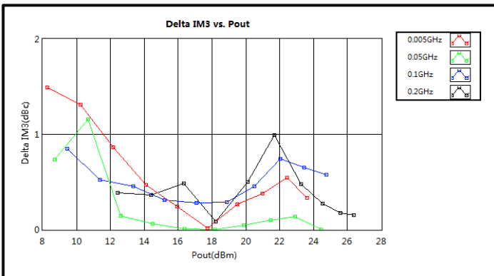
Delta IM3 vs. Pout (5MHz-200MHz)
