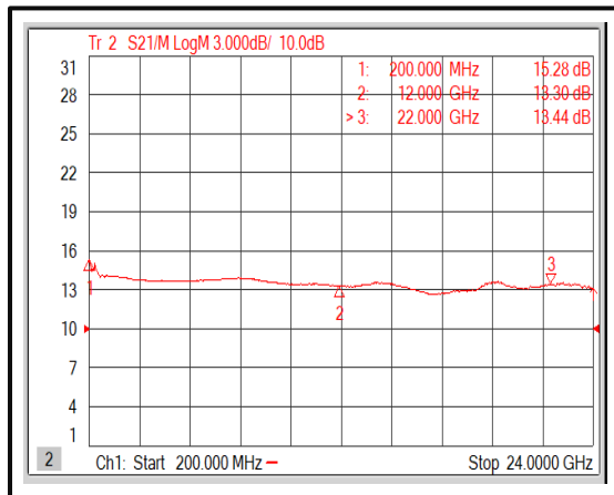
Gain@+25°C (200MHz-22GHz)
