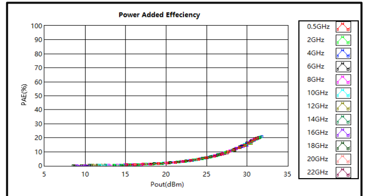
Power Added Efficiency (0.5GHz-22GHz)
