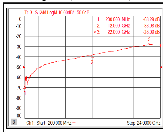
Isolation@+85°C (200MHz-22GHz)
