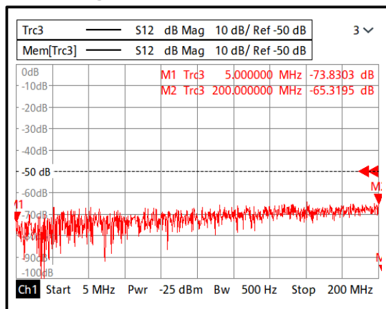
Isolation@+85°C (5MHz-200MHz)
