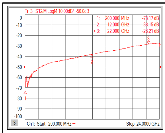
Isolation@+25°C (200MHz-22GHz)
