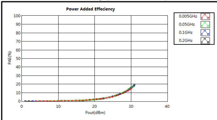
Power Added Efficiency (5MHz-200MHz)
