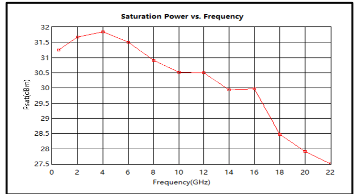
Saturation Power vs. Frequency (0.5GHz-22GHz)
