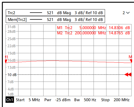
Gain@+85°C (5MHz-200MHz)
