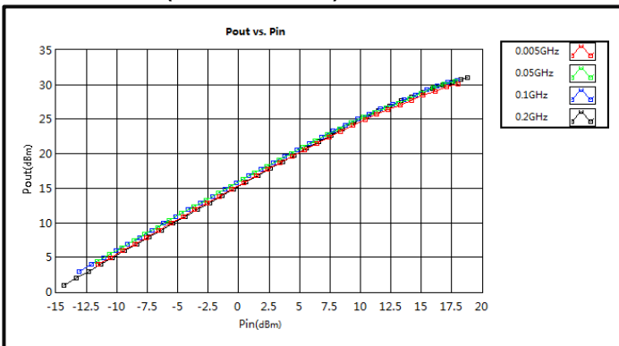
Pout vs. Pin (5MHz-200MHz)
