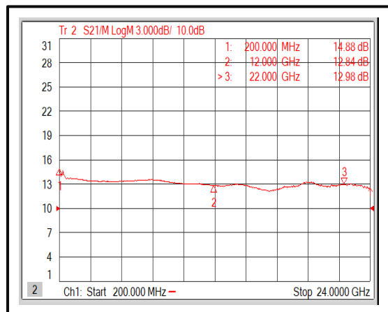
Gain@+85°C (200MHz-22GHz)
