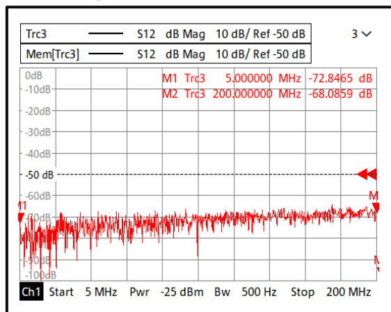
Isolation@+25°C (5MHz-200MHz)
