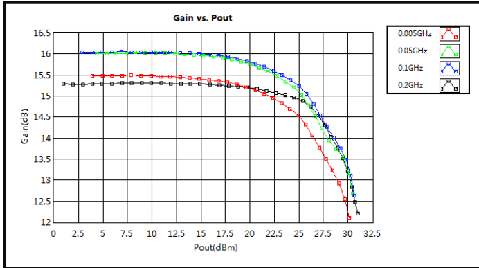
Gain vs. Output Power (5MHz-200MHz)
