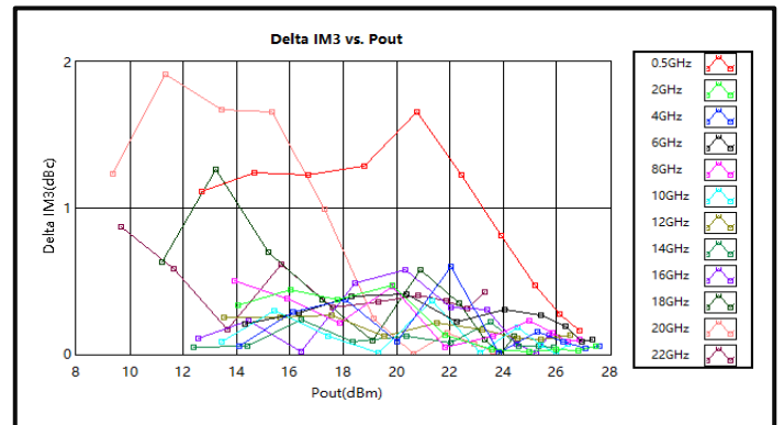
Delta IM3 vs. Pout (0.5GHz-22GHz)
