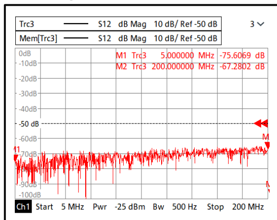
Isolation@-40°C (5MHz-200MHz)
