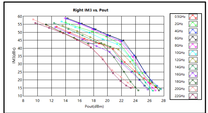
Right IM3 vs. Pout (0.5GHz-22GHz)
