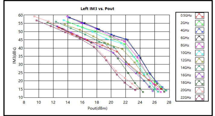
Left IM3 vs. Pout (0.5GHz-22GHz)
