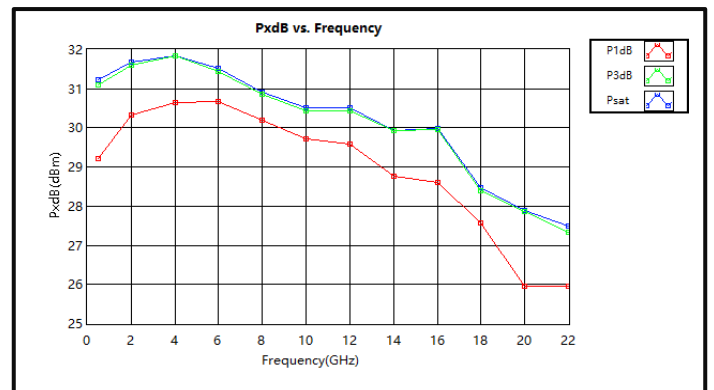
PndB vs. Frequency (0.5GHz-22GHz)
