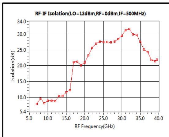
RF-IF Isolation
