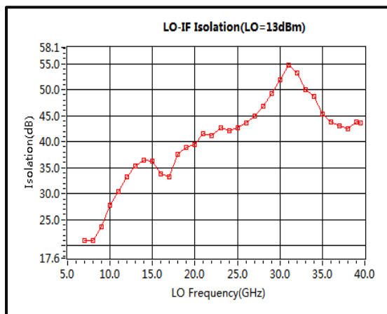
LO-IF Isolation
