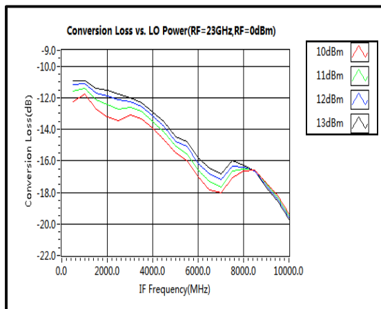
Conversion Loss vs. LO Power
