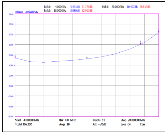
Noise Figure (4GHz-20GHz)
