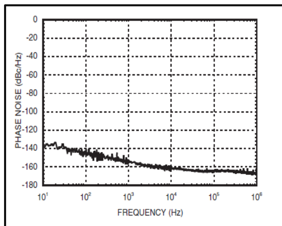
Phase Noise @ 12GHz
