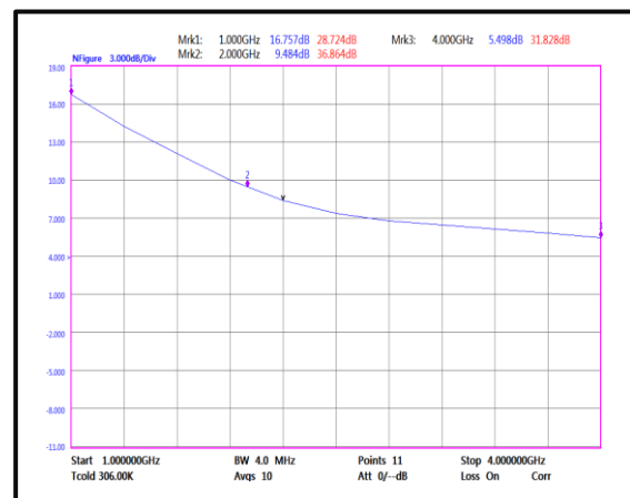
Noise Figure (1GHz-4GHz)
