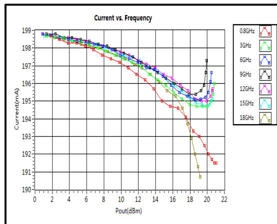
Current vs. Frequency
