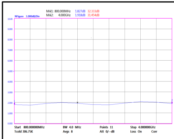
Noise Figure (0.8GHz-4GHz)
