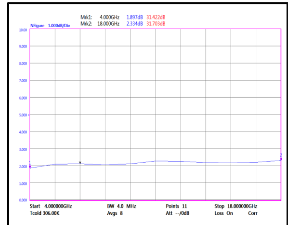
Noise Figure (4GHz-18GHz)
