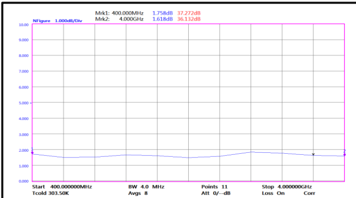
Noise Figure (0.4GHz-4GHz)
