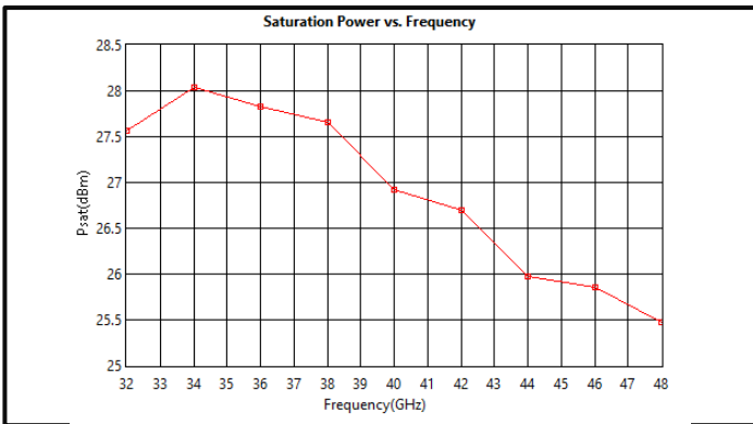
Psat vs Frequency
