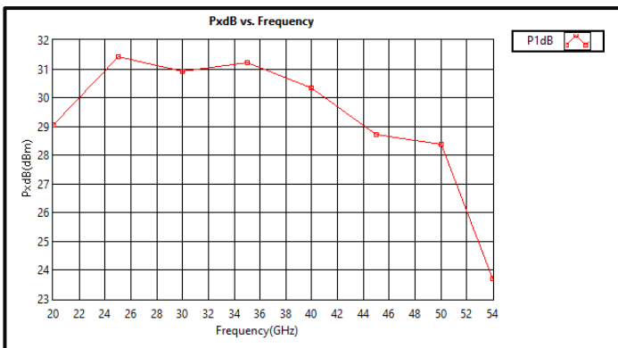
PxdB vs Frequency @ +25°C
