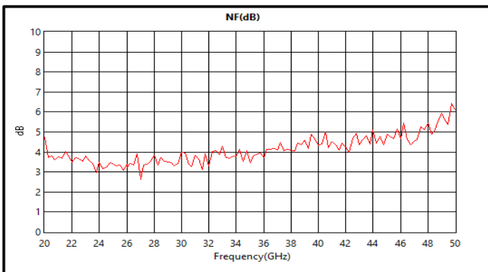
Noise Figure vs Frequency @ +25°C
