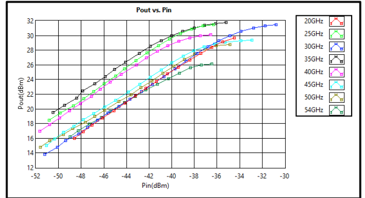
Output vs Input Power @ +25°C
