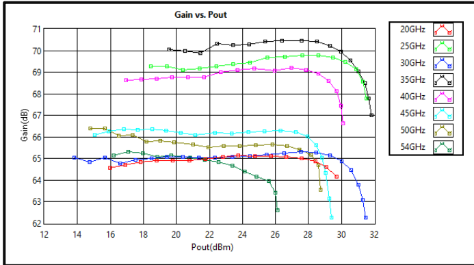
Gain vs Output Power @ +25°C
