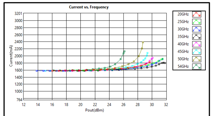
Current vs Output Power (+12VDC) @ +25°C
