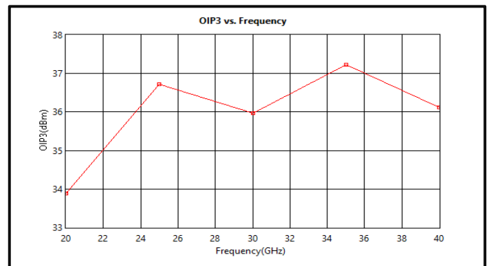
OIP3 vs Frequency @ +25°C
