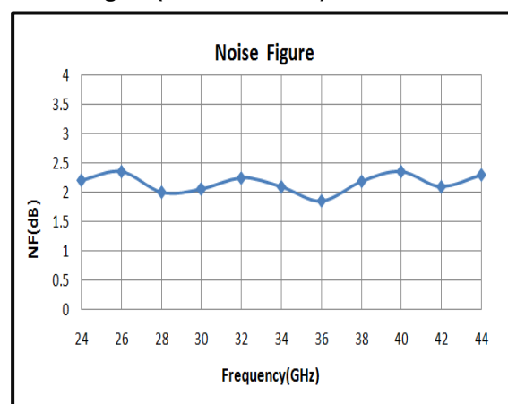
Noise Figure(24GHz-44GHz)
