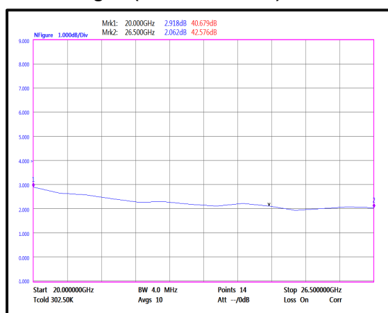
Noise Figure(20GHz-26.5GHz)
