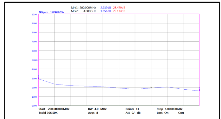
Noise Figure(200MHz-4GHz)
