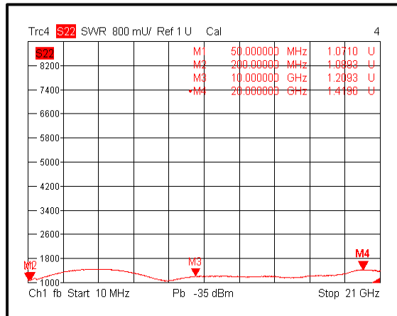
Output VSWR@+25°C
