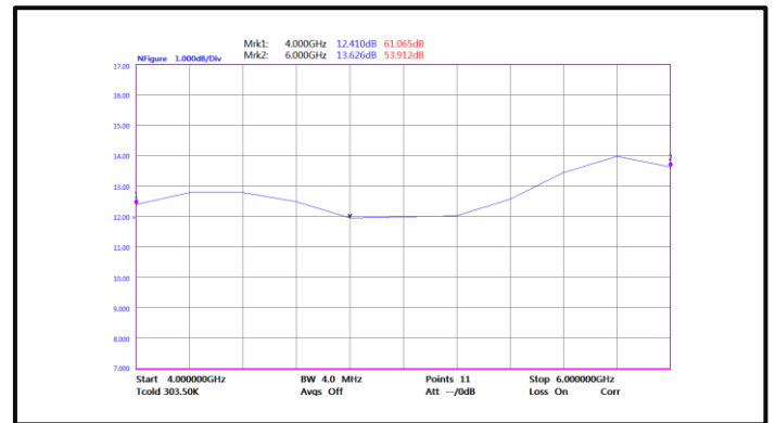
Noise Figure(4GHz-6GHz)
