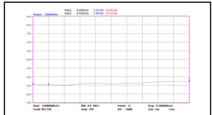
Noise Figure(4GHz-4.5GHz)
