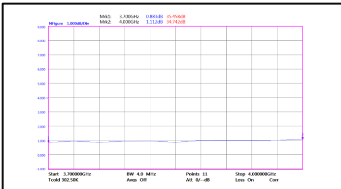
Noise Figure(3.7GHz-4GHz)
