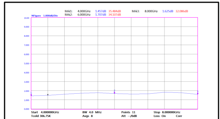
Noise Figure (4GHz-8GHz)
