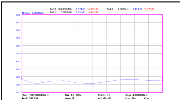
Noise Figure (0.5GHz-4GHz)
