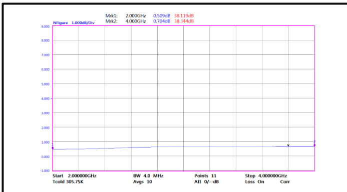
Noise Figure(2-4GHz)
