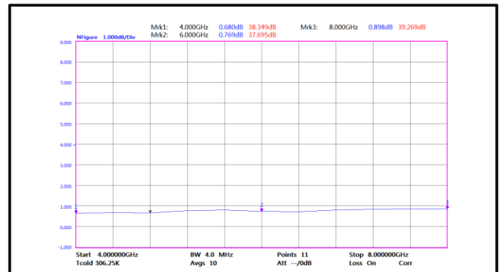
Noise Figure(4-8GHz)
