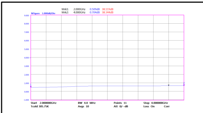
Noise Figure(2-4GHz)
