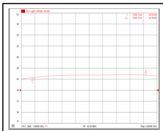
Gain@+85°C
