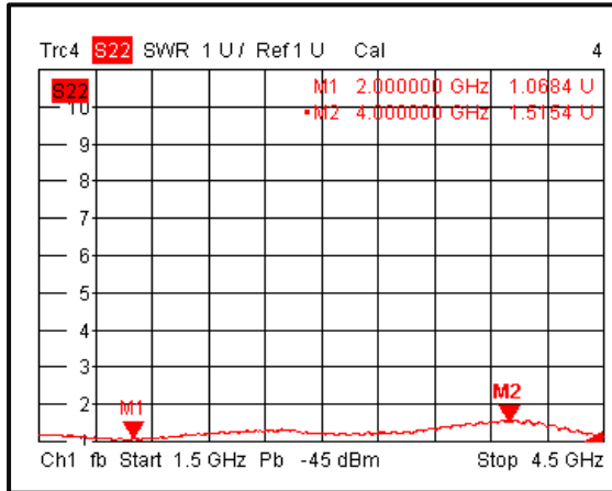
Output VSWR@+25°C
