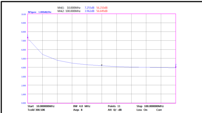
Noise Figure(0.01GHz-0.1GHz)
