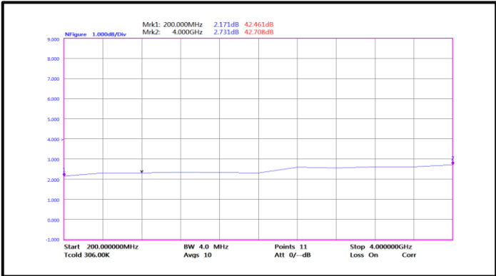
Noise Figure(0.2GHz-4GHz)
