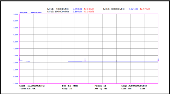
Noise Figure(0.01GHz-0.2GHz)
