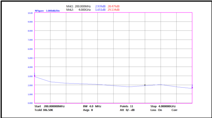
Noise Figure(200MHz-4GHz)
