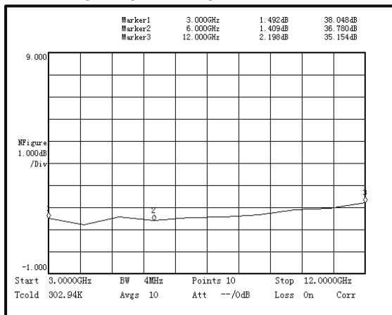
Noise Figure (3-12GHz)
