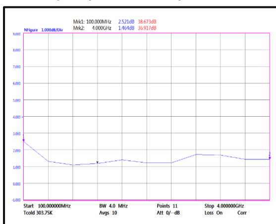
Noise Figure (100MHz-4GHz)
