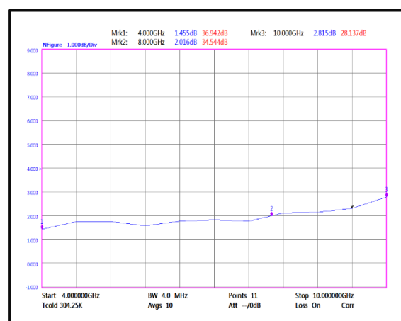
Noise Figure (4GHz-10GHz)
