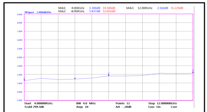
Noise Figure (4GHz-12GHz)
