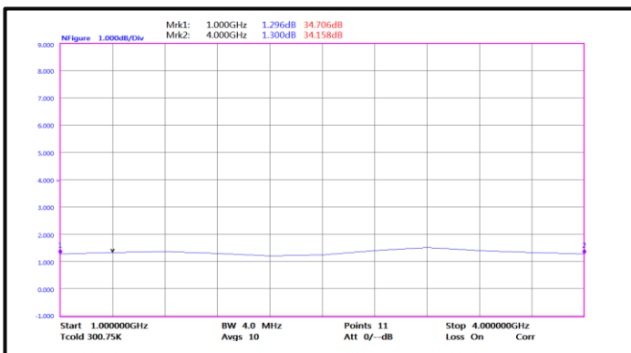
Noise Figure (1GHz-4GHz)
