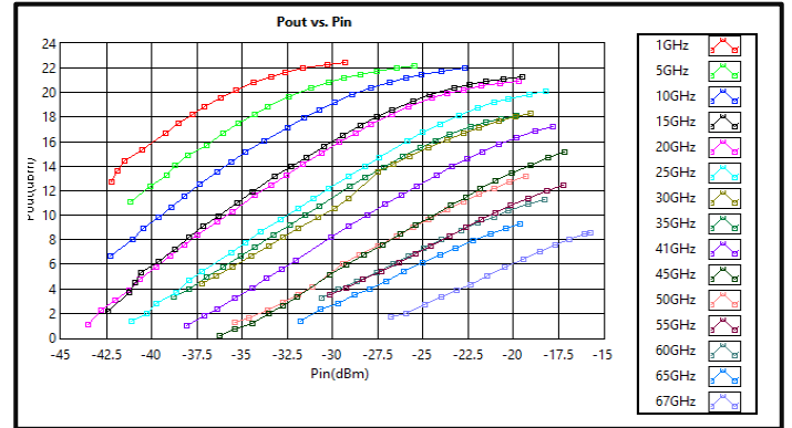
Output vs Input Power @ +85°C
