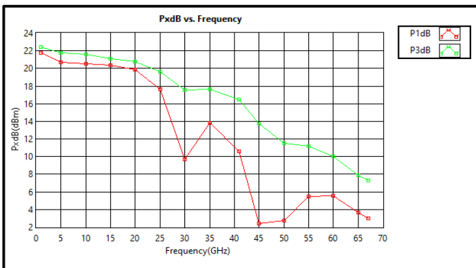
PxdB vs Frequency @ +85°C
