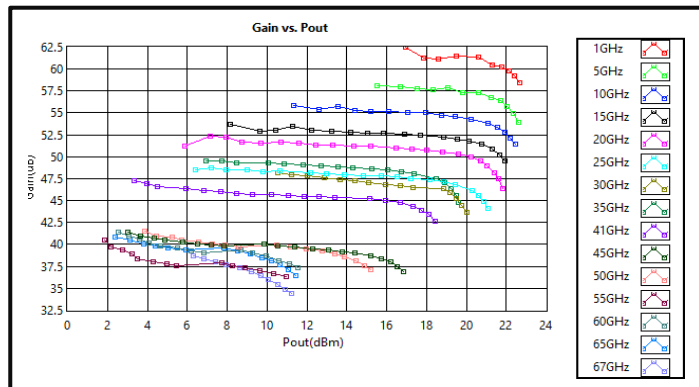
Gain vs Output Power @ -40°C
