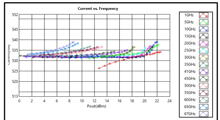
Current vs Output Power (+12VDC) @ +85°C
