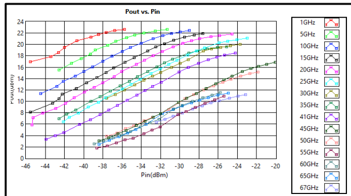
Output vs Input Power @ -40°C
