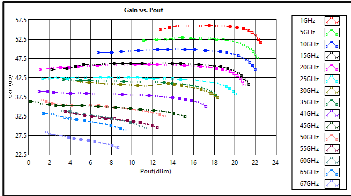
Gain vs Output Power @ +85°C
