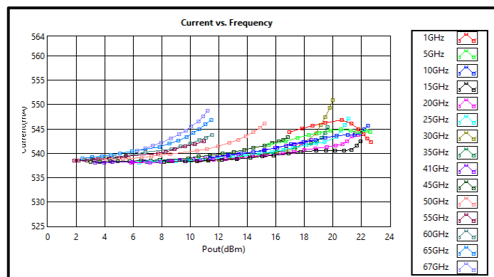
Current vs Output Power (+12VDC) @ -40°C
