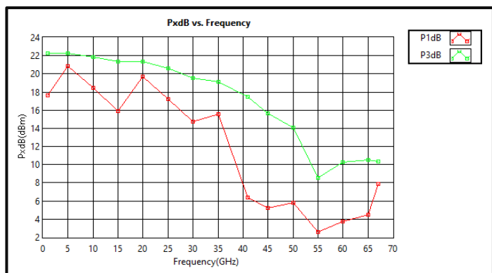
PxdB vs Frequency @ -40°C
