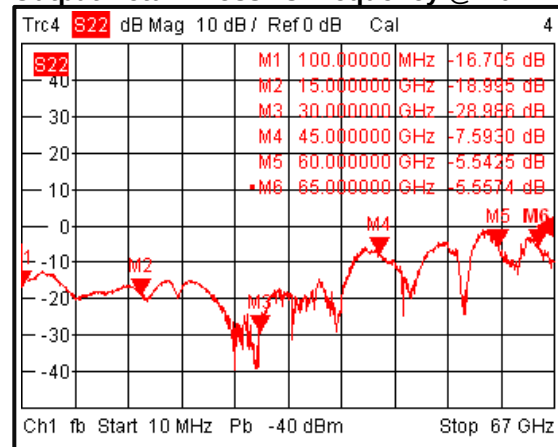
Output Return Loss vs Frequency @-40°C
