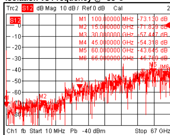
Isolation vs Frequency @+85°C
