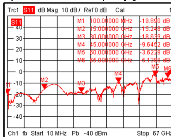
Input Return Loss vs Frequency @-40°C
