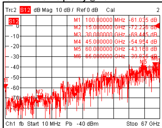
Isolation vs Frequency @-40°C
