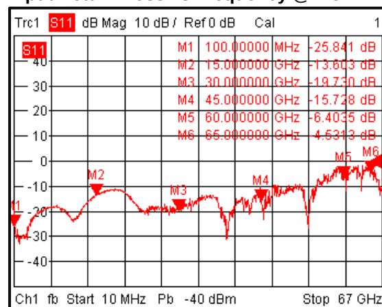
Input Return Loss vs Frequency @+25°C
