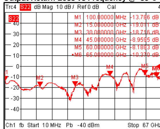
Output Return Loss vs Frequency @+85°C
