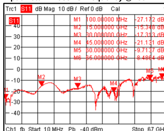
Input Return Loss vs Frequency @+85°C
