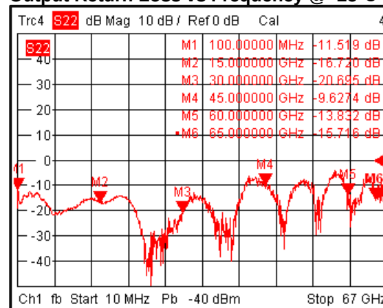
Output Return Loss vs Frequency @+25°C
