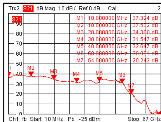
Gain vs. Frequency @-10°C
