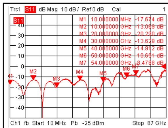
Input Return Loss vs Frequency @-10°C
