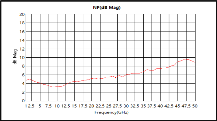
Noise Figure (1GHz-50GHz)
