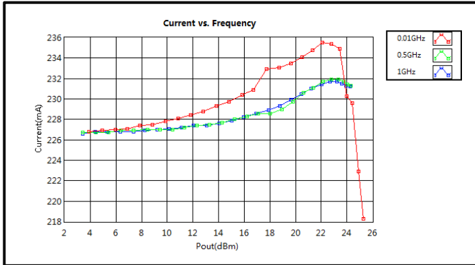
Current vs. Pout (0.01GHz-1GHz)
