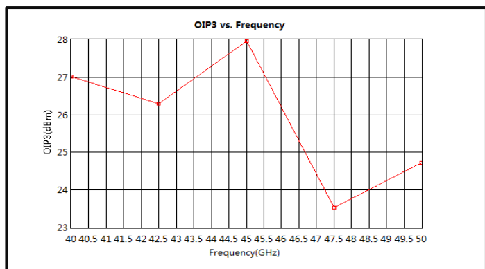
Output Third Order Intercept (OIP3) (40GHz-50GHz)
