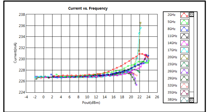
Current vs. Pout (2GHz-38GHz)
