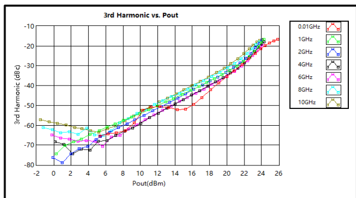
3rd Harmonic Wave Output Power (0.01GHz-10GHz)
