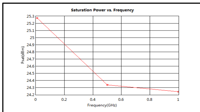
Saturation Power vs. Frequency (0.01GHz-1GHz)
