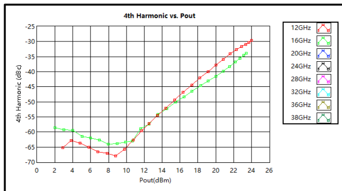
4th Harmonic Wave Output Power (12GHz-38GHz)
