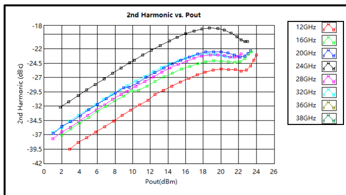
2nd Harmonic Wave Output Power (12GHz-38GHz)
