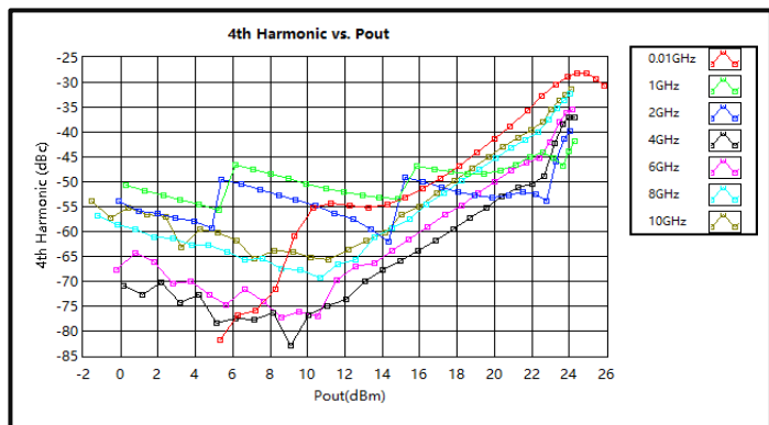
4th Harmonic Wave Output Power (0.01GHz-10GHz)
