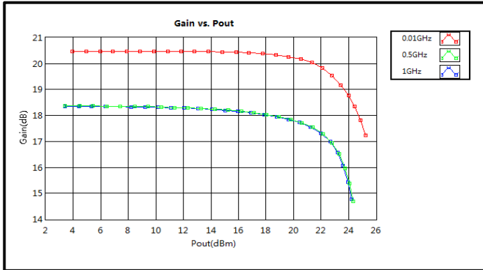
Gain vs. Output Power (0.01GHz-1GHz)
