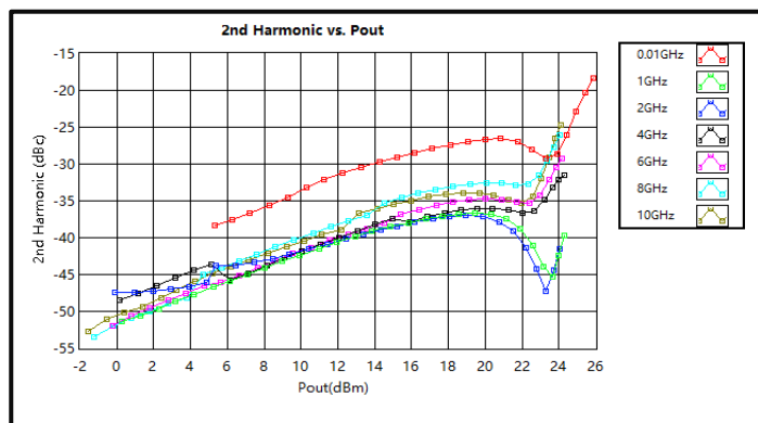
2nd Harmonic Wave Output Power (0.01GHz-10GHz)
