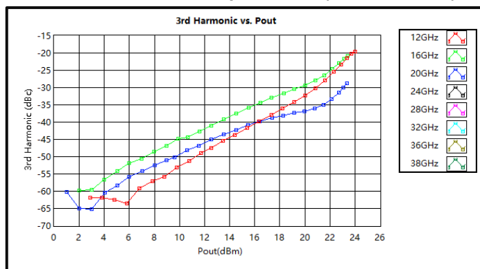
3rd Harmonic Wave Output Power (12GHz-38GHz)
