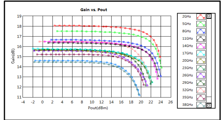
Gain vs. Output Power (2GHz-38GHz)
