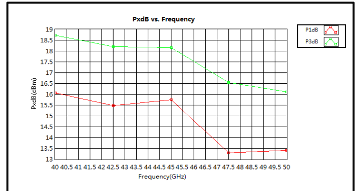
P1dB & P3dB vs. Frequency (40GHz-50GHz)
